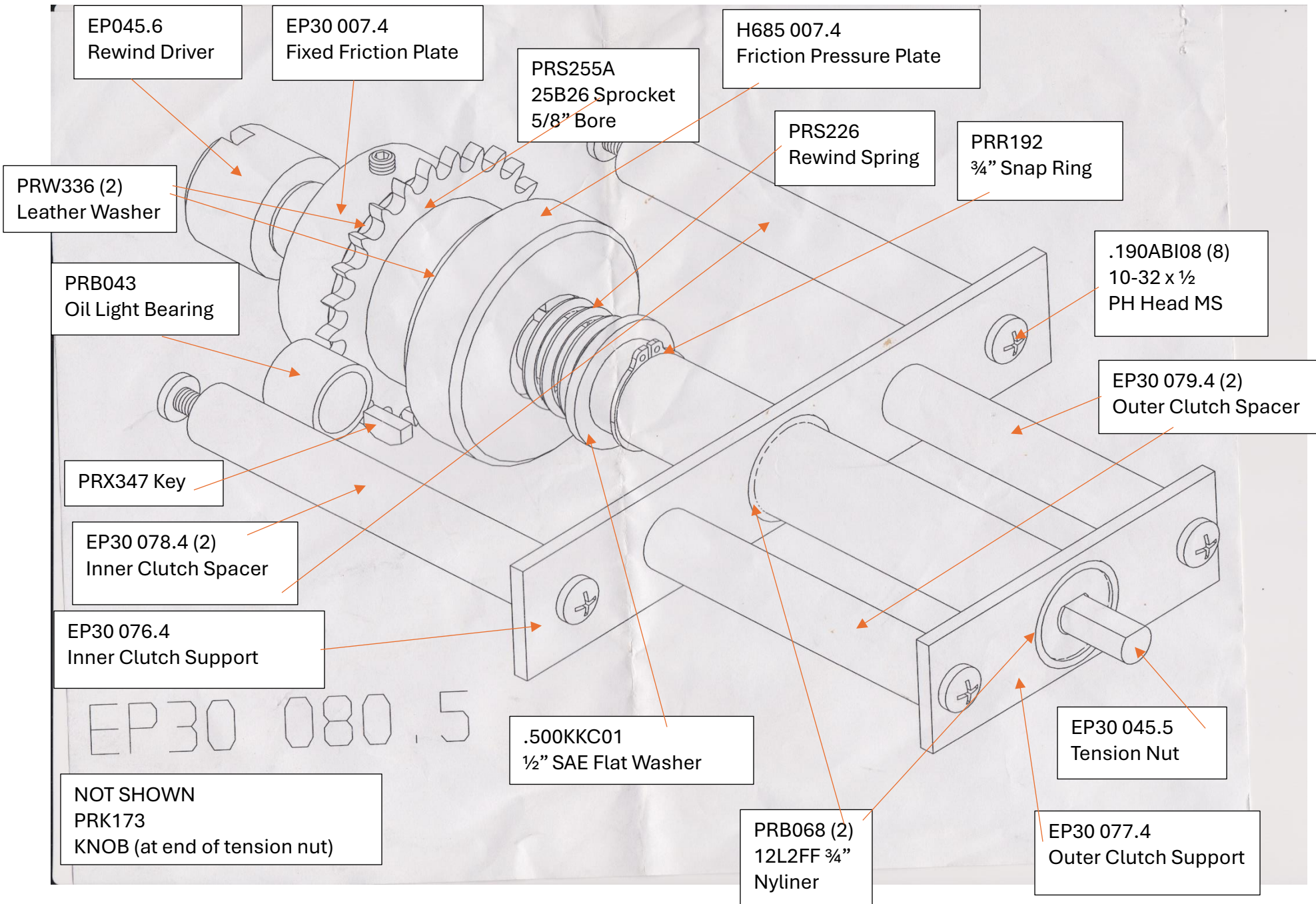
EP30 080.5 ASSEMBLY. FOR ECONCRAFT (EP30,44,50,60) AND HRD44 AND EHR44 LAMINATORS
